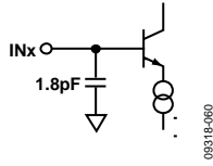
Figure 58. Analog Input
