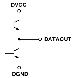
Figure 64. Logic Output
