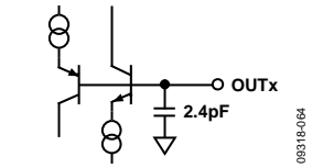
Figure 62. Analog Output Disabled
