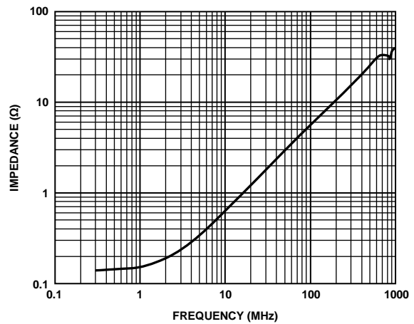
Figure 41. ADV3229 Output Impedance, Enabled
