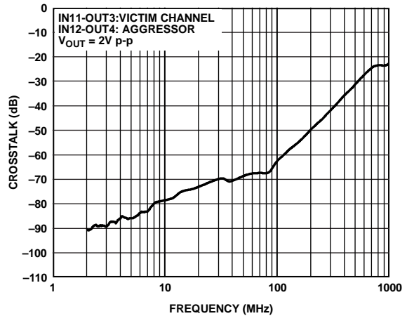
Figure 34. ADV3229 Crosstalk, One Adjacent Channel, RTO
