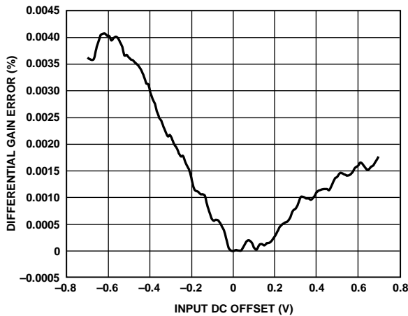
Figure 45. ADV3228 Differential Gain Error
