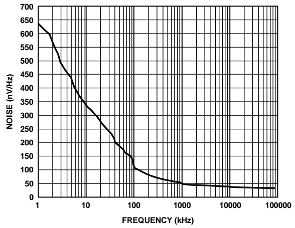
Figure 29. ADV3229 Output Noise, 100 Ω Load
