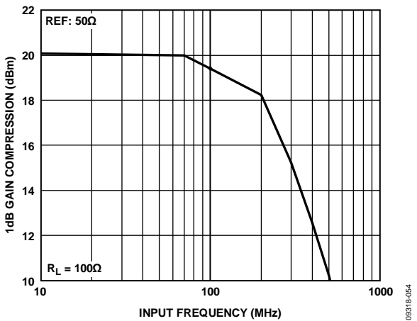
Figure 51. ADV3229 1 dB Gain Compression, 100 \Omega Load
