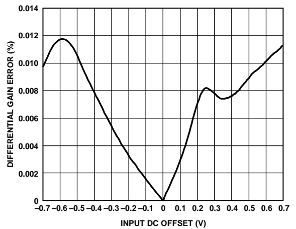
Figure 48. ADV3229 Differential Gain Error
