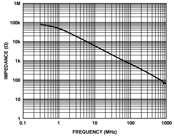
Figure 40. ADV3229 Output Impedance, Disabled
