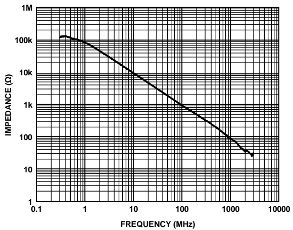
Figure 36. ADV3229 Input Impedance
