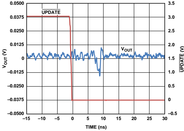
Figure 43. ADV3228 Switching Glitch
