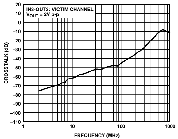
Figure 35. ADV3229 Crosstalk, All Hostile, RTO
