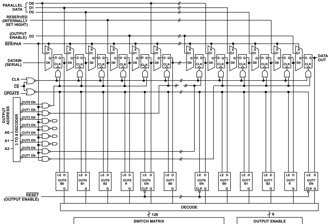
Figure 6. Logic Diagram
