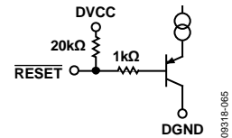
Figure 63. Reset Input
