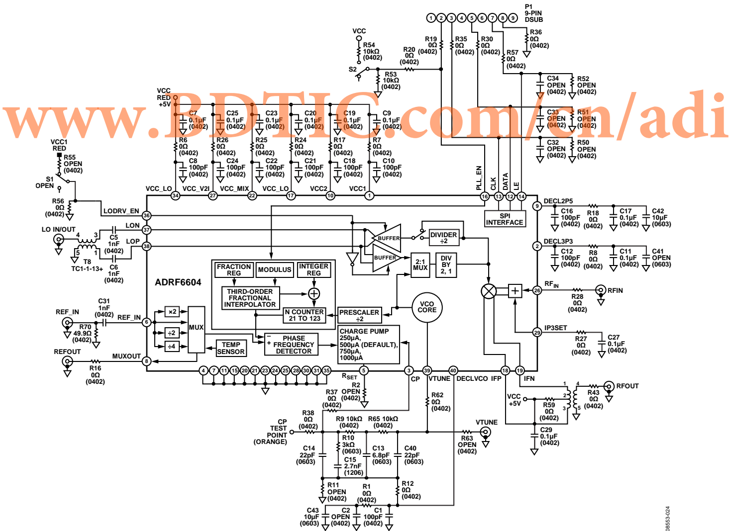
Figure 46. Basic Connections for Operation of the ADRF6604
