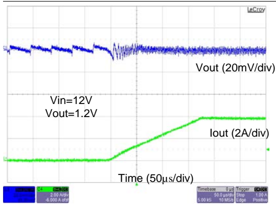
Figure 17. Transition from DCM to CCM Operation
