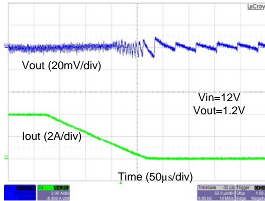
Figure 18. Transition from CCM to DCM Operation
