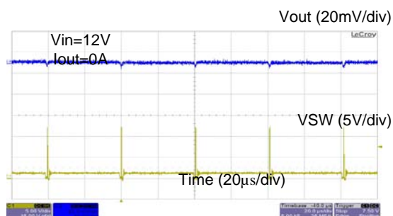
Figure 15. Static Load Ripple at Light-Load
