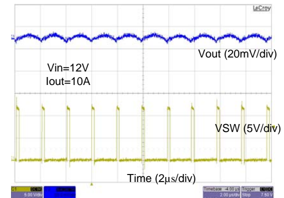
Figure 16. Static Load Ripple at Full Load
