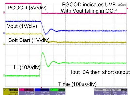
Figure 21. Over-Current Protection with Heavy Load Applied
