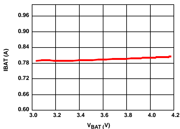
FIGURE 4. CHARGE CURRENT vs OUTPUT VOLTAGE
