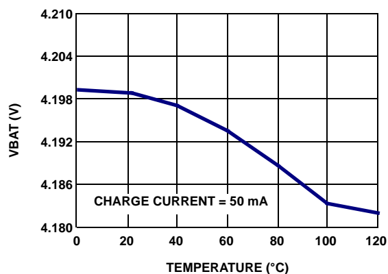
FIGURE 2. CHARGER OUTPUT VOLTAGE vs TEMPERATURE
