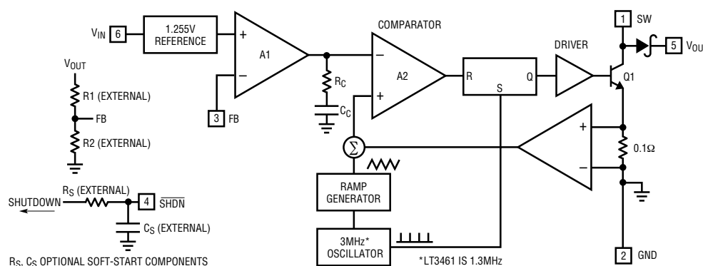
Figure 1. Block Diagram
