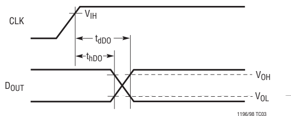
Figure 3. Voltage Waveform for D_{OUT} Delay Time, t_{dDO} and t_{hDO}
