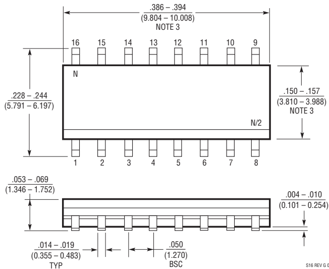
S Package 16-Lead Plastic Small Outline (Narrow .150 Inch) (Reference LTC DWG # 05-08-1610 Rev G)
