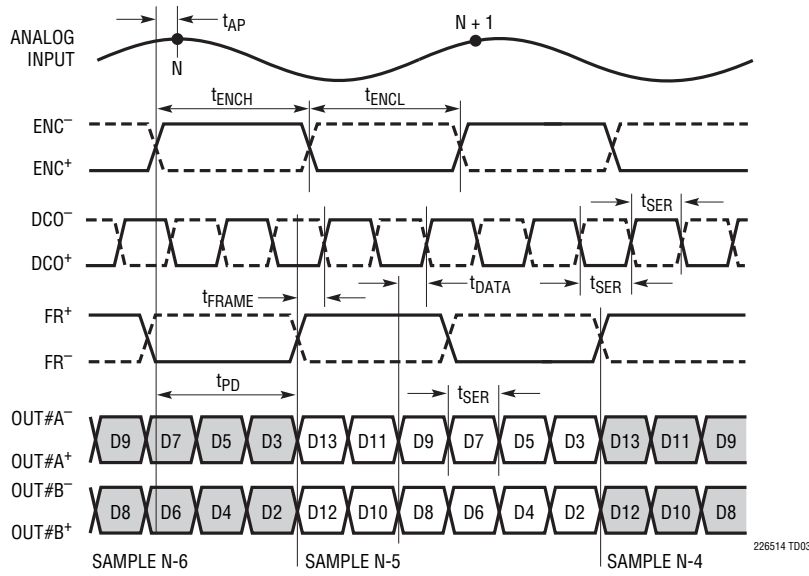
2-Lane Output Mode, 12-Bit Serialization
