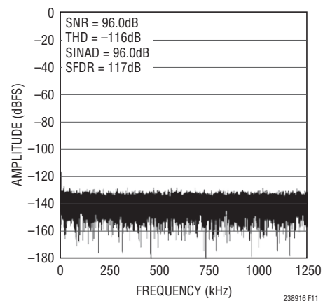
Figure 11. 32k Point FFT of LTC2389-16, f_{\text{SAMPL}} = 2.5\text{Mps} , f_{\text{IN}} = 2\text{kHz}
