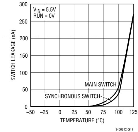
Switch Leakage vs Temperature
