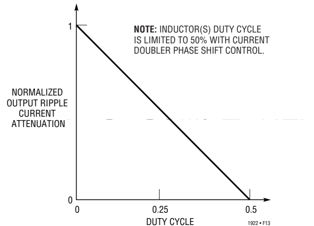
Figure 15. Ripple Current Cancellation vs Duty Cycle
