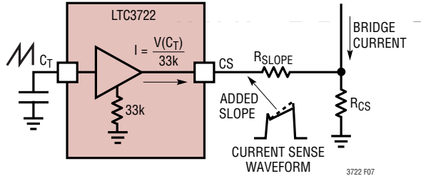
Figure 9. Slope Compensation Circuitry
