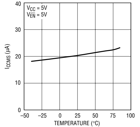
Manual Shutdown Supply Current vs Temperature
