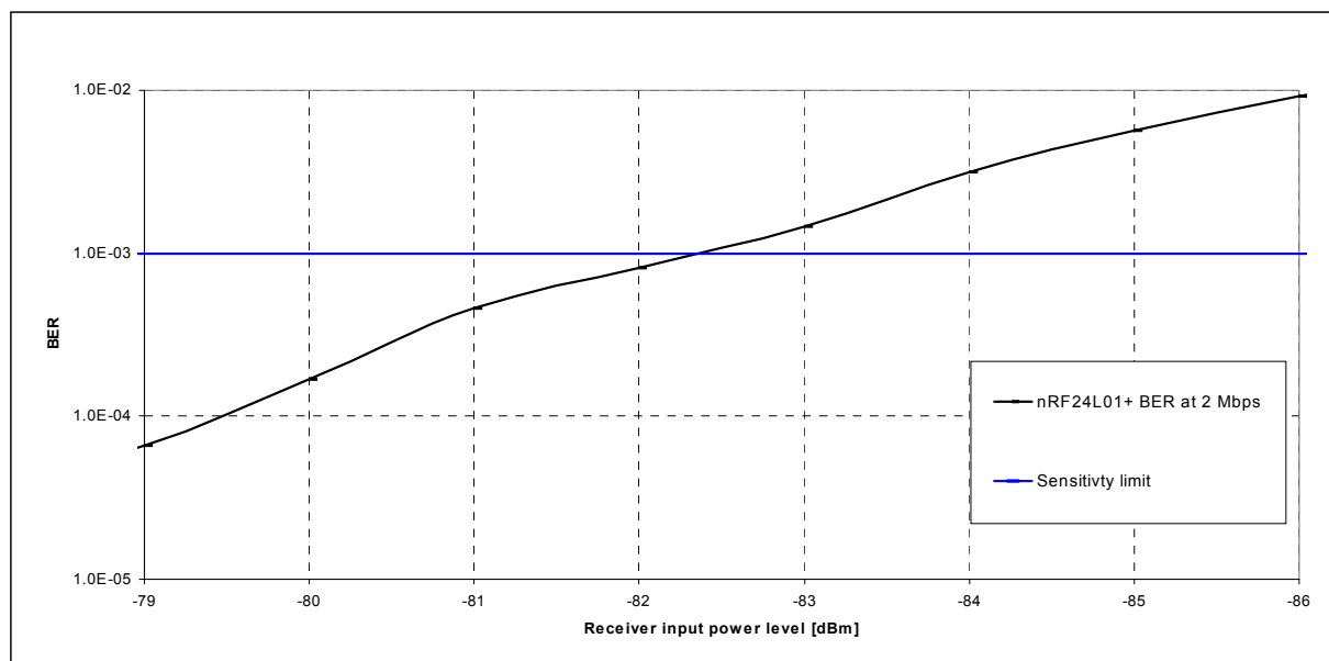
Figure 17. nRF24L01+ BER vs. RF input power
