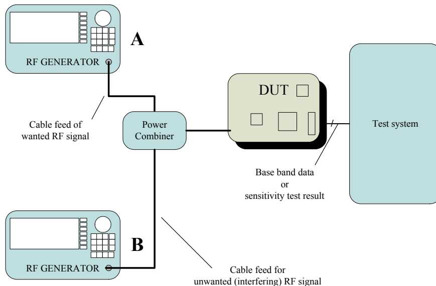
Figure 23. RX selectivity test setup
