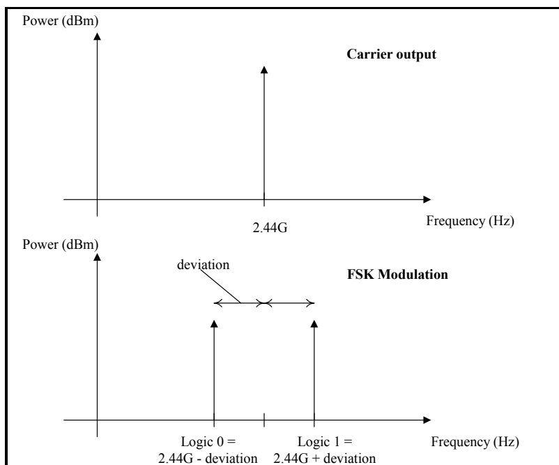
Figure 11. FSK modulation
