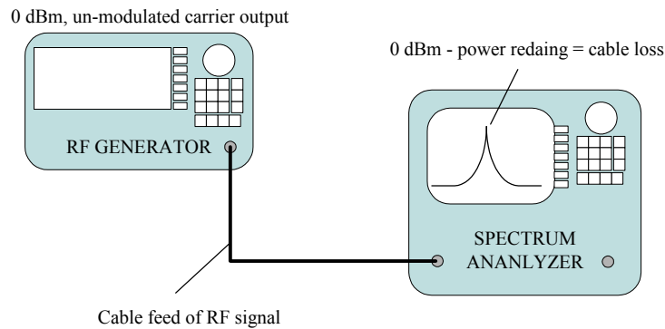
Figure 20. Calibrating DUT power input
