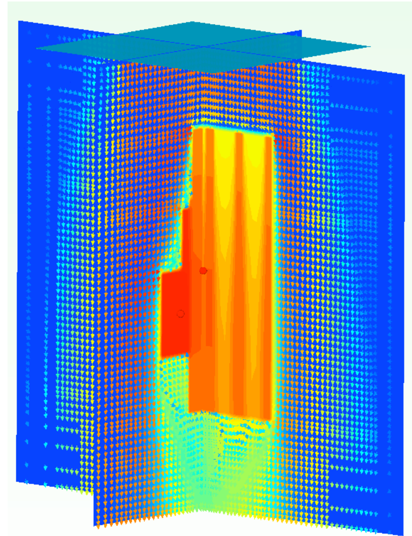
Option 1 Air flow direction
