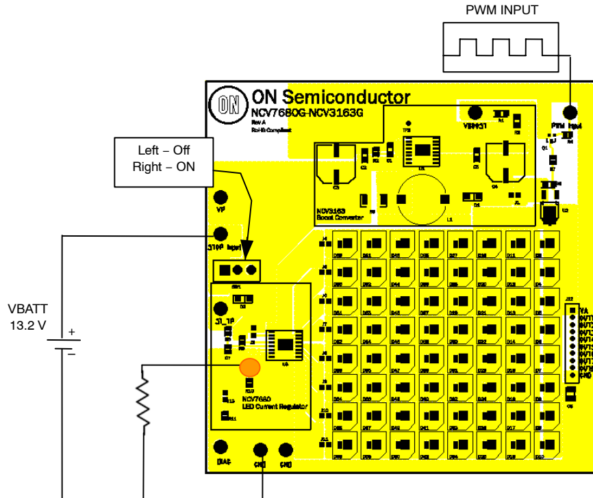
Figure 7. RSTOP Programming Resistor
