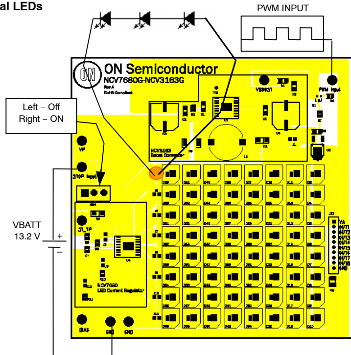
Figure 10. Additional LEDs (Only One Strand Shown)
