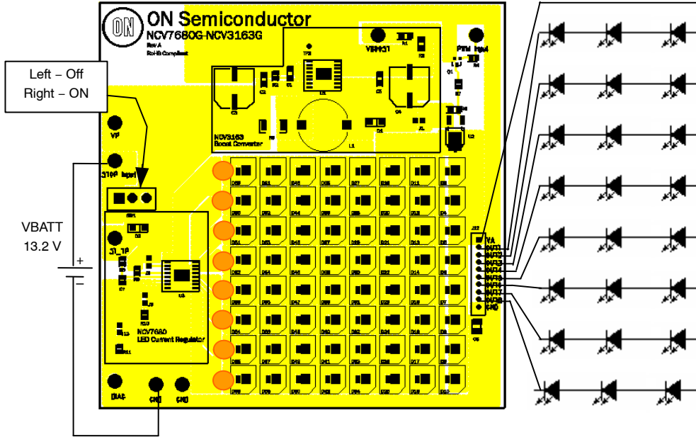
Figure 9. External LEDs
