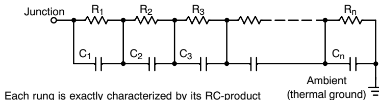
Figure 13. Non-Grounded Capacitor Thermal Ladder ("Foster" Ladder)
