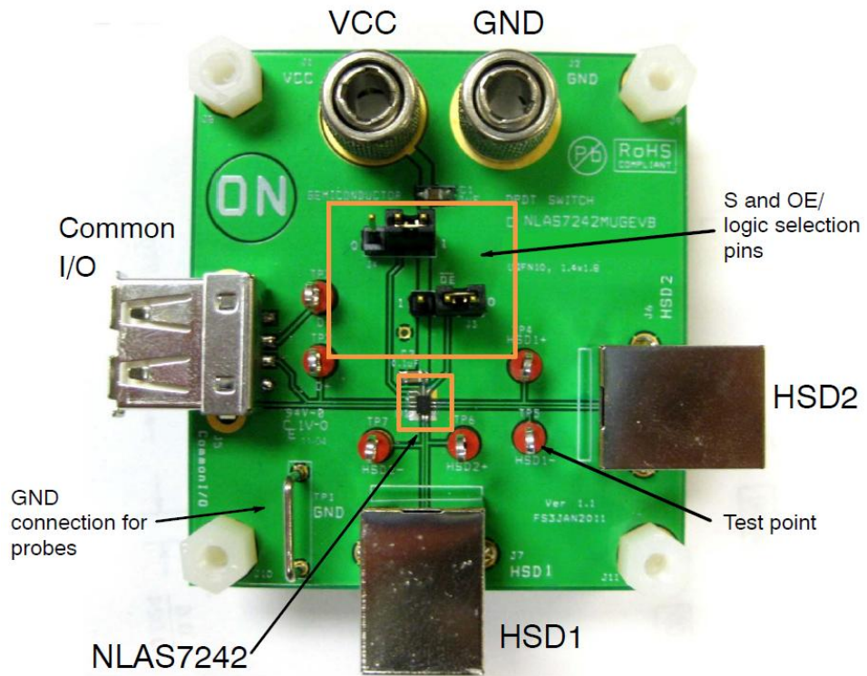
Figure 1. Demo Board Close-Up
