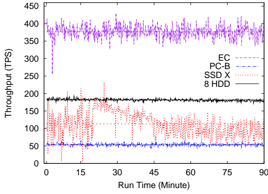
Figure 4: Variation in Transaction Throughput
