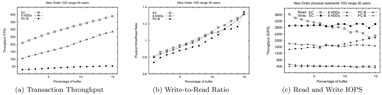
Figure 3: Write-to-Read Ratio and Buffer Size
