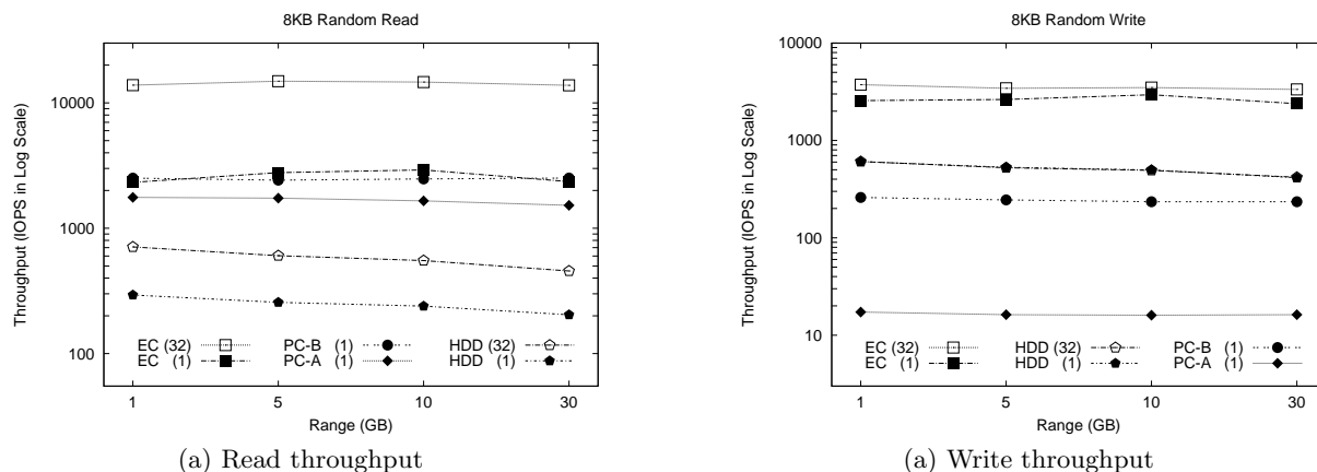
Figure 1: Small Random I/O Throughput vs. Data Access Range
