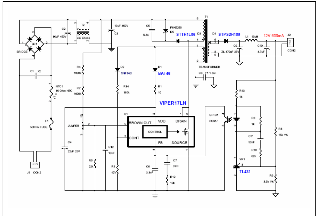
Figure 1. EVALVIPER17L-7W schematic
