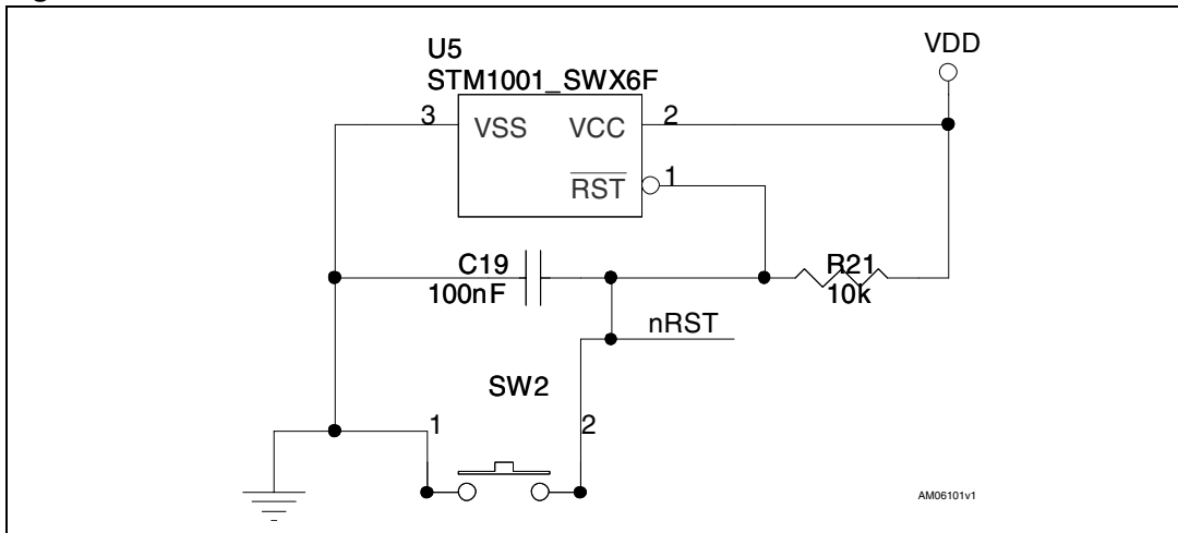
Figure 7. Reset section
