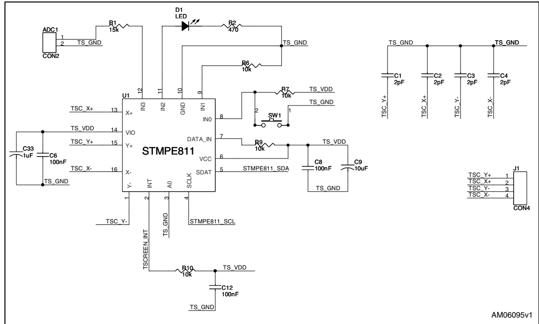
Figure 1. Touchscreen controller
