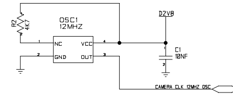
CAMERA OSCILLATOR
