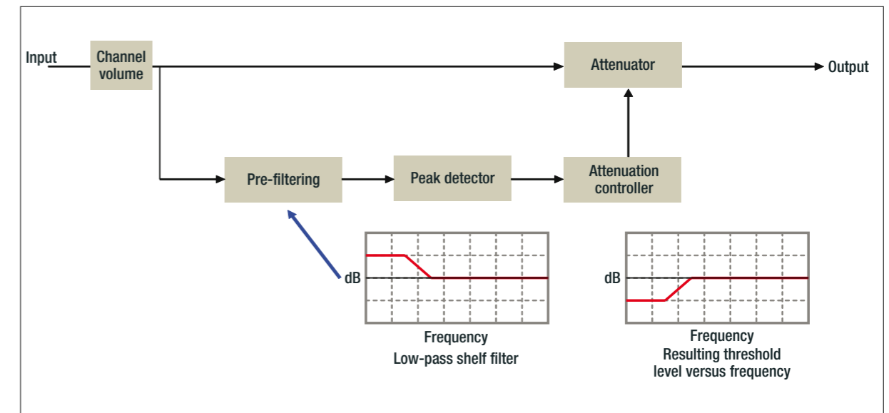
Figure 3: EqDRC block diagram
