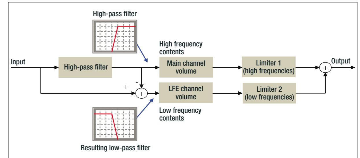
Figure 2: Dual-band DRC (depicted for a single channel only)
