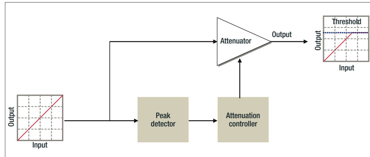
Figure 1: Limiter in DRC or anti-clipping
