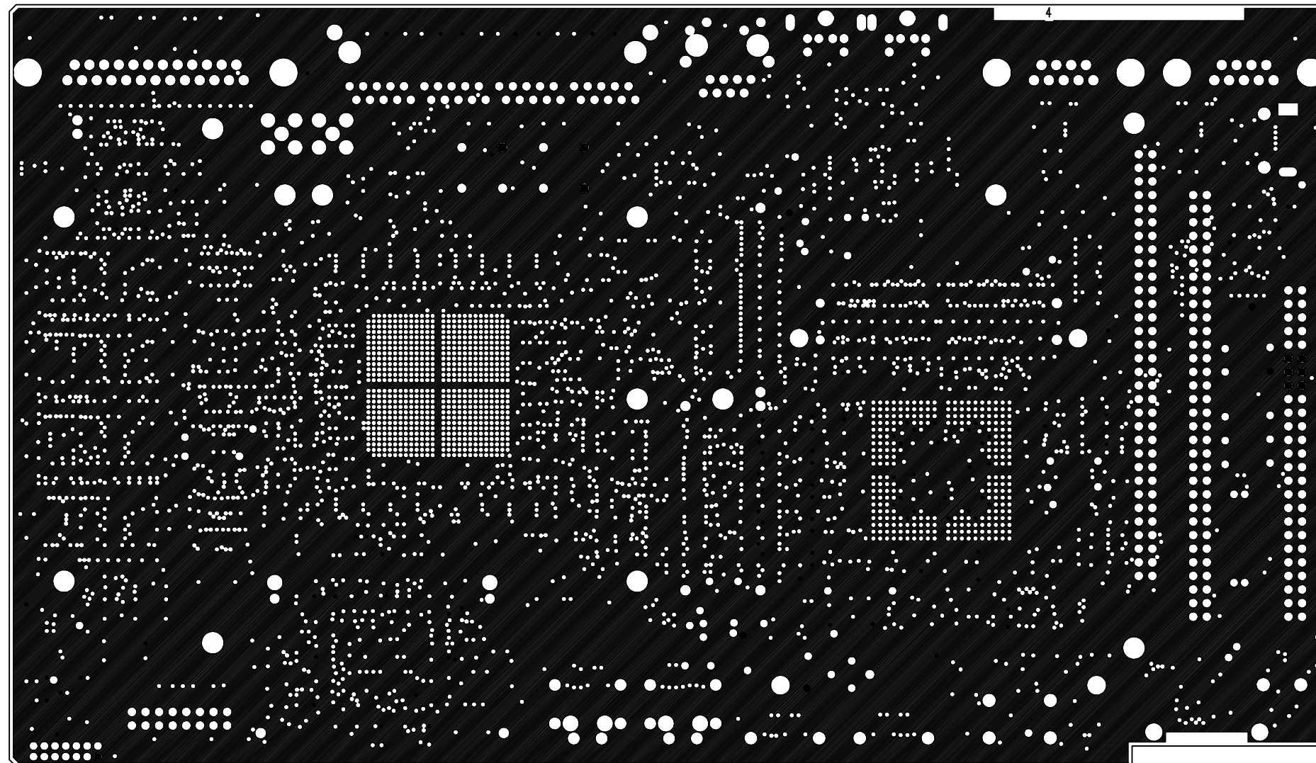
VCC3.3 Plane (L4)
