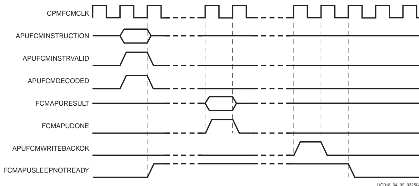
Figure 4-10: APU Controller Decoded Store Instruction with StoreWBOK=1
