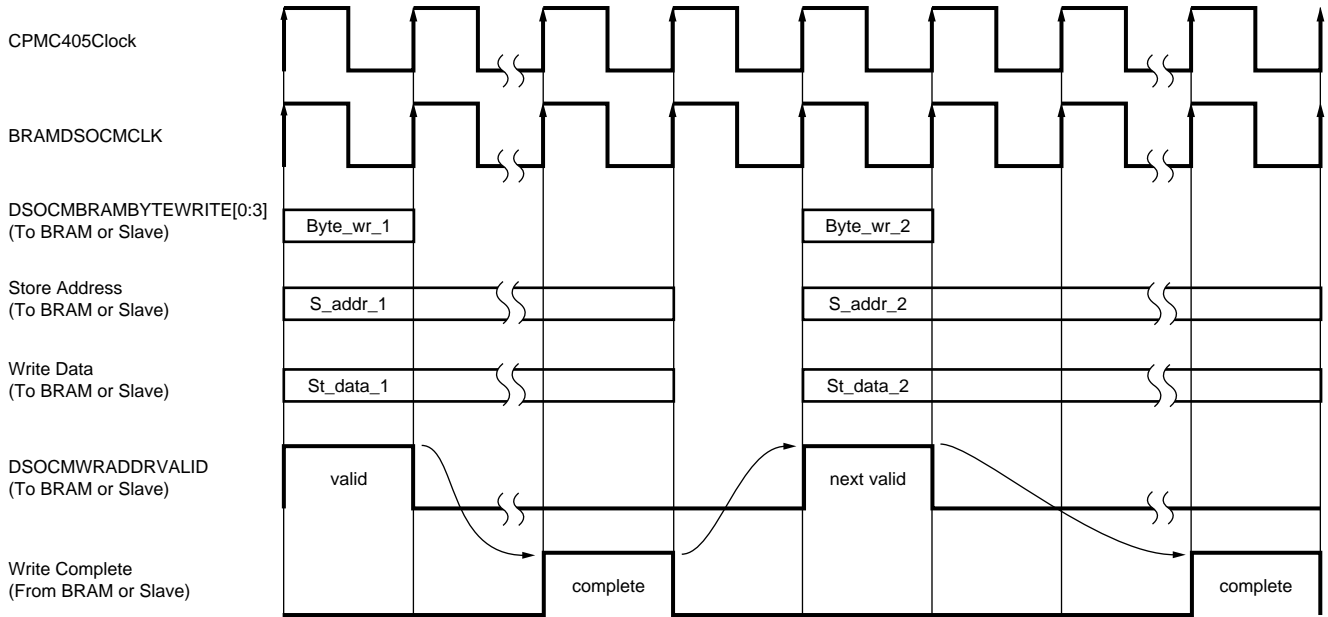
Figure 3-28: Single Cycle Mode (1:1) DSOCM Write Variable Latency Virtex-4
