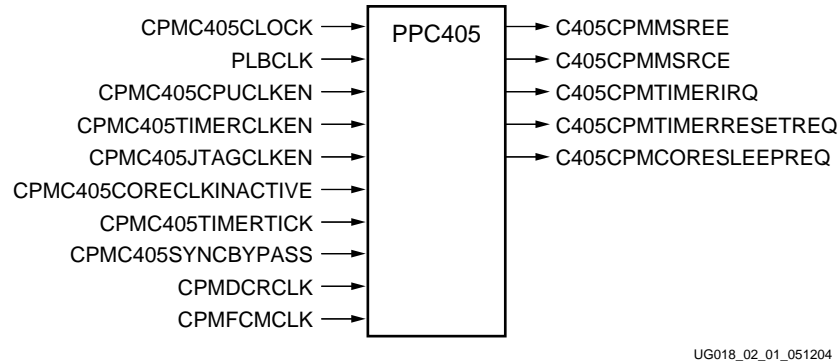
Figure 2-1: CPM Interface Block Symbol
