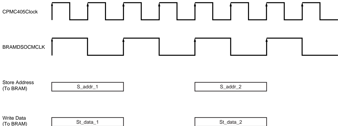
Figure 3-25: Multi Cycle Mode (2:1) Data Store Timing
