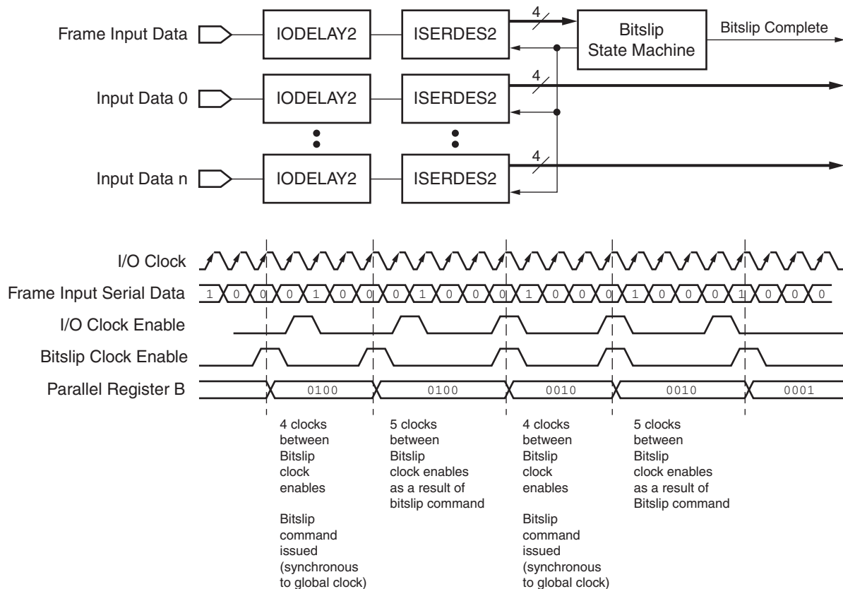
Figure 3-3: Bit Slip Timing Diagram of ISERDES2 Block (4:1 illustrated)
