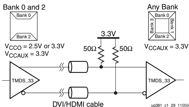
Figure 1-19: External Input Resistors Required for TMD5_33 I/O Standard
