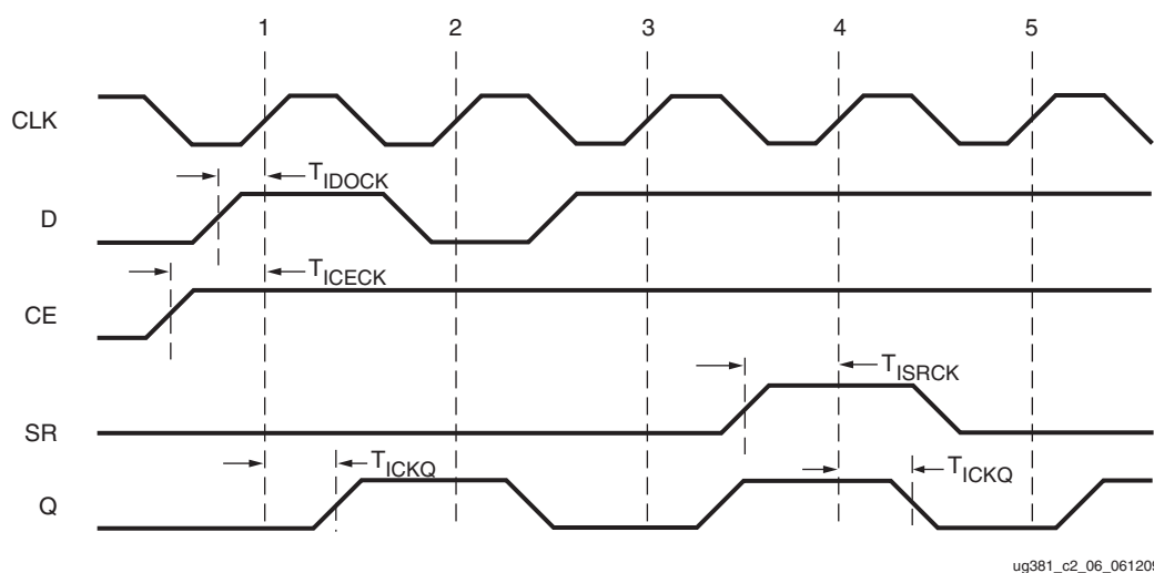
Figure 2-8: ILOGIC2 Input Register Timing Characteristics
