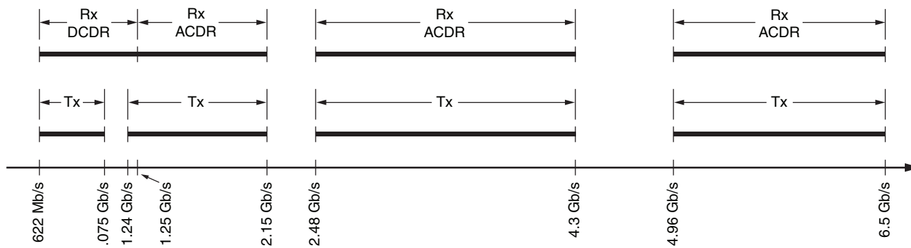
Figure 1: Transmitter and Receiver Line Rates
