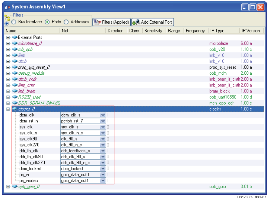
Figure 5: System Assembly View / Ports Filter, Clock Module Connections
