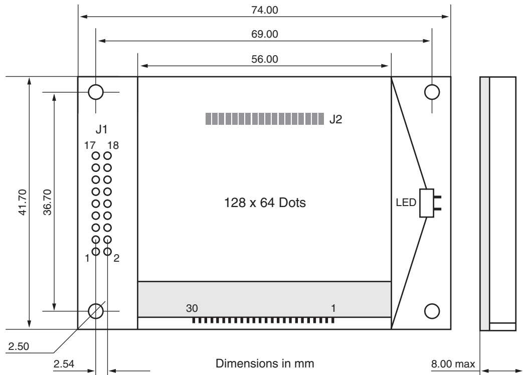
Figure 3-5: 64128EFCBC-3LP Dimensions
