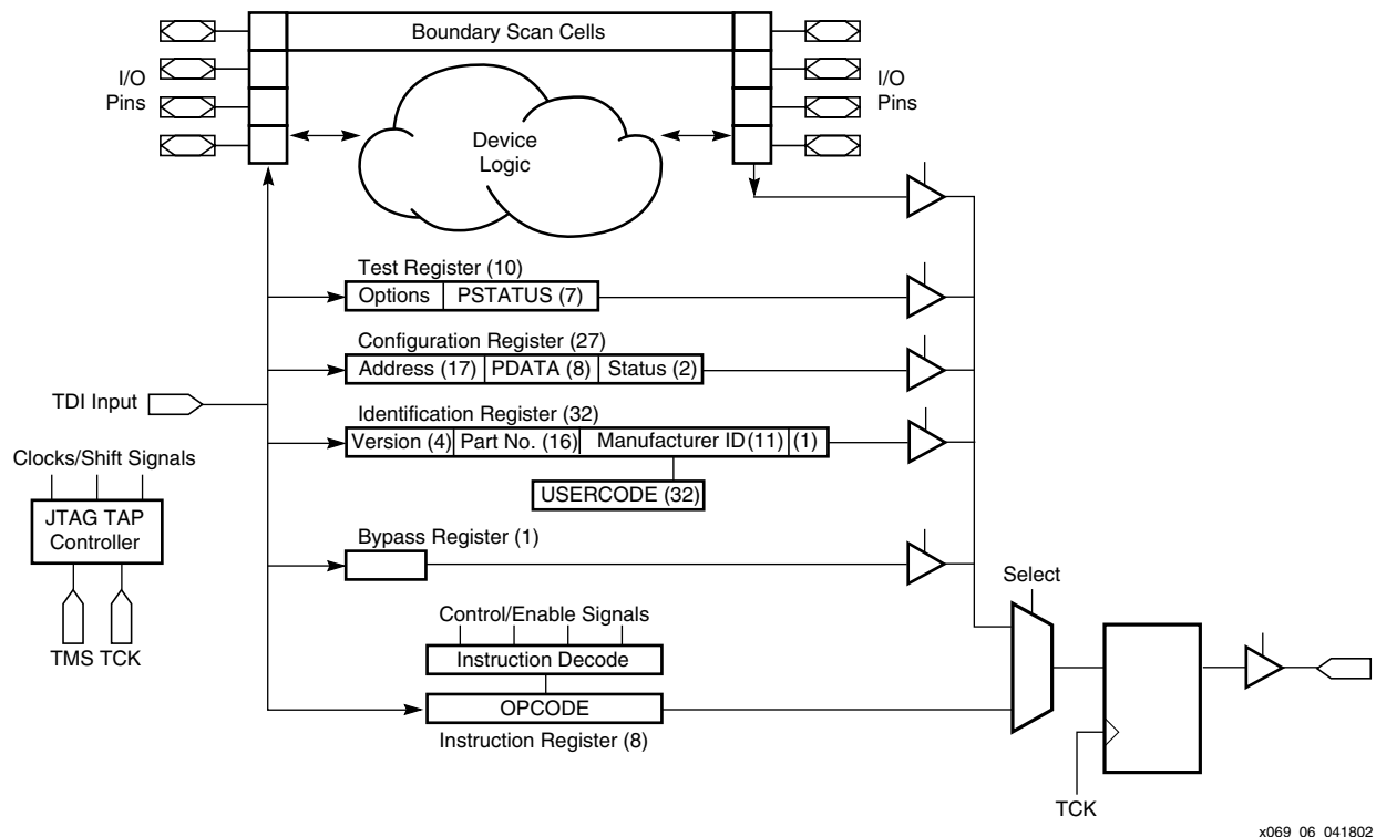
Figure 6: JTAG Architecture
