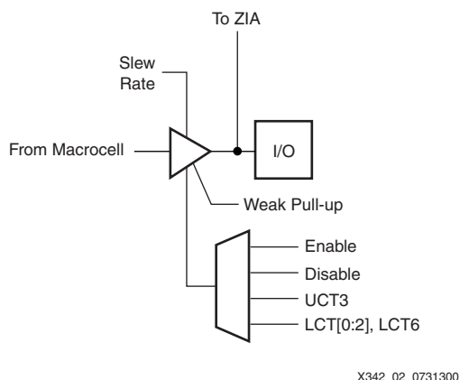
Figure 2: Input/Output Cell Architecture
