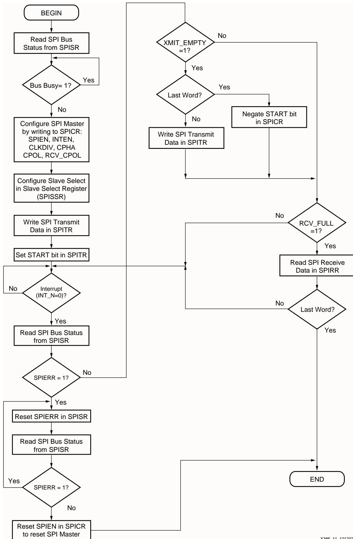
Figure 11: CoolRunner-II SPI Master Transaction Flow Chart
