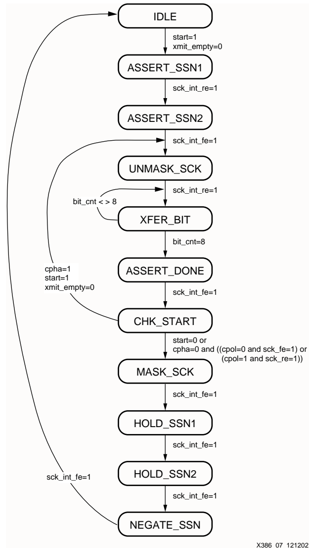
Figure 7: SPI Control State Machine
