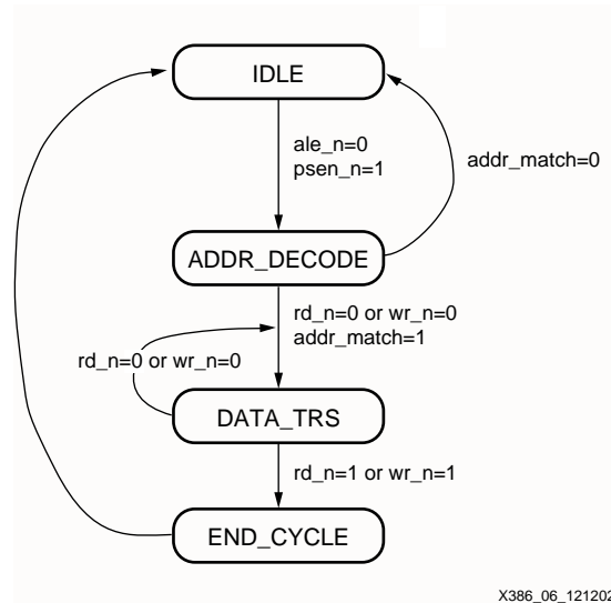
Figure 6: \mu C Bus Interface State Machine
