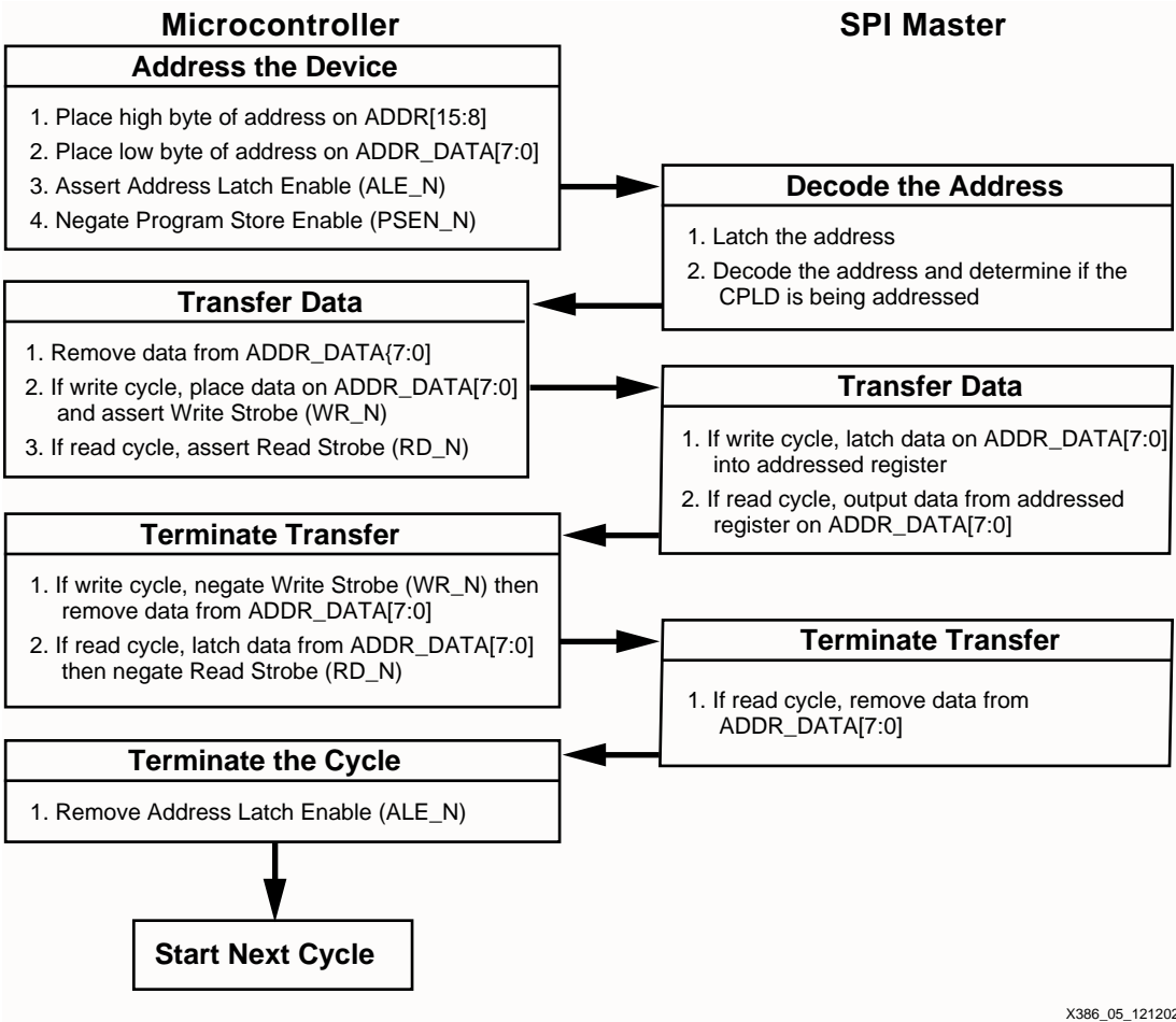
Figure 5: µC Read/Write Protocol
