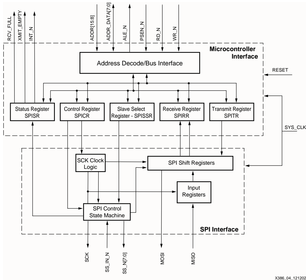
Figure 4: SPI Master Block Diagram
