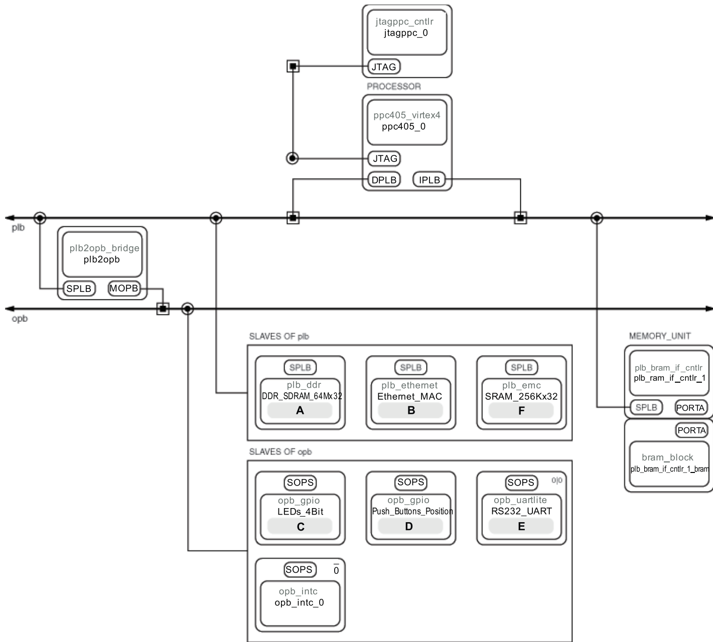
Figure 1: PowerPC Web Server Design
