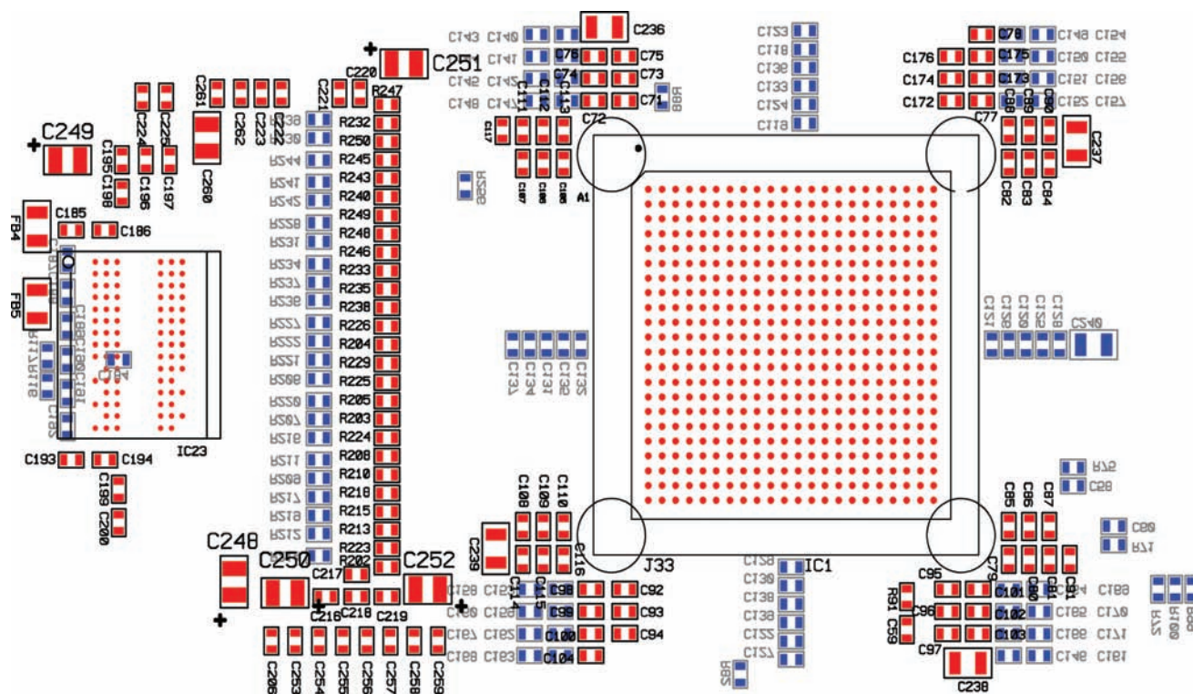
Figure 5: Component Placement
