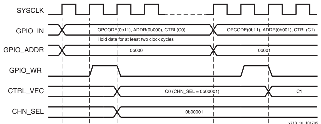
Figure 10: Timing Diagram of GPIO Write on the Multi-Channel XBERT Module
