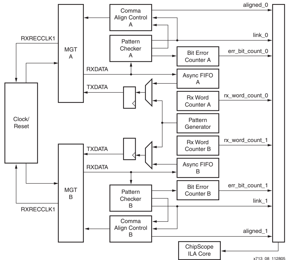
Figure 8: Single-Channel XBERT Module
