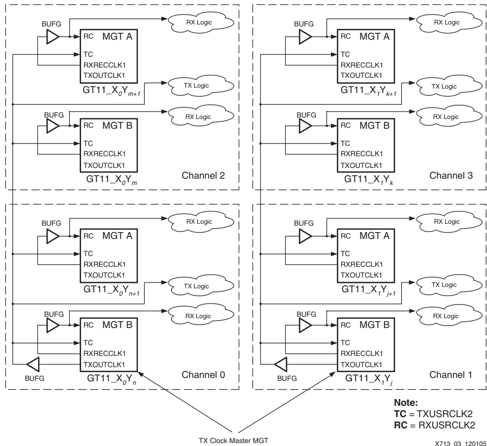
Figure 3: MGT User Clock Distribution in XBERT Reference Design
