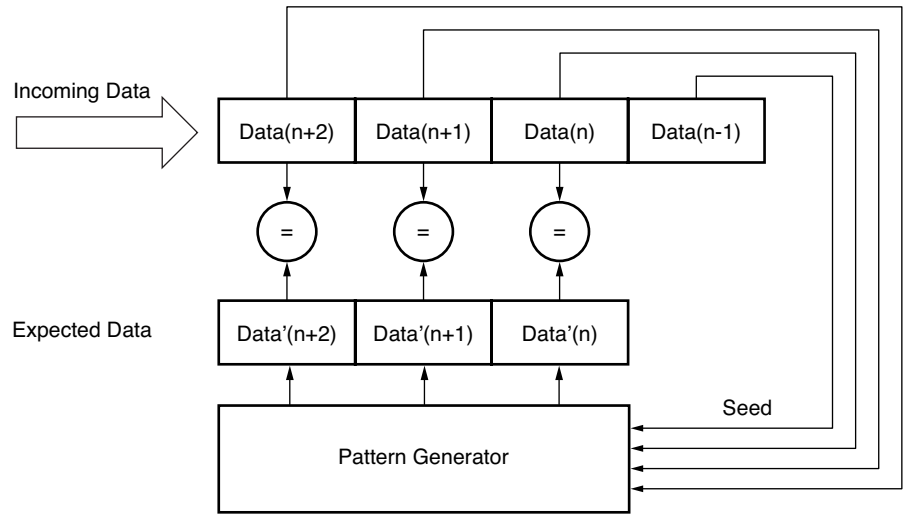
Figure 6: Self Synchronized Pattern Checker
