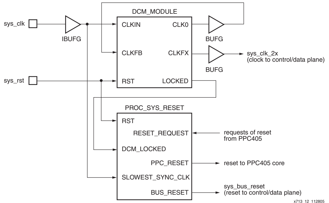
Figure 12: Clock and Reset Distribution in the Control Plane
