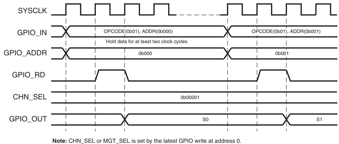
Figure 11: Timing Diagram of GPIO Read on the Multi-Channel XBERT Module
