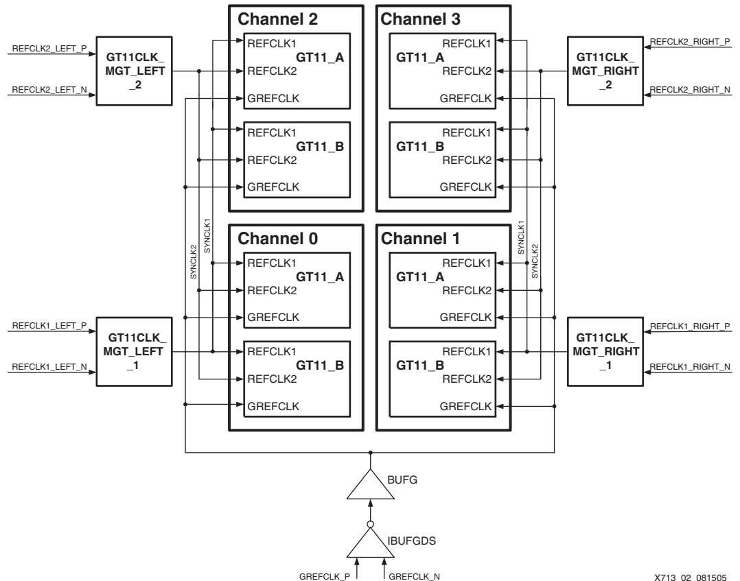
Figure 2: MGT Reference Clock Distribution in XBERT Reference Design
