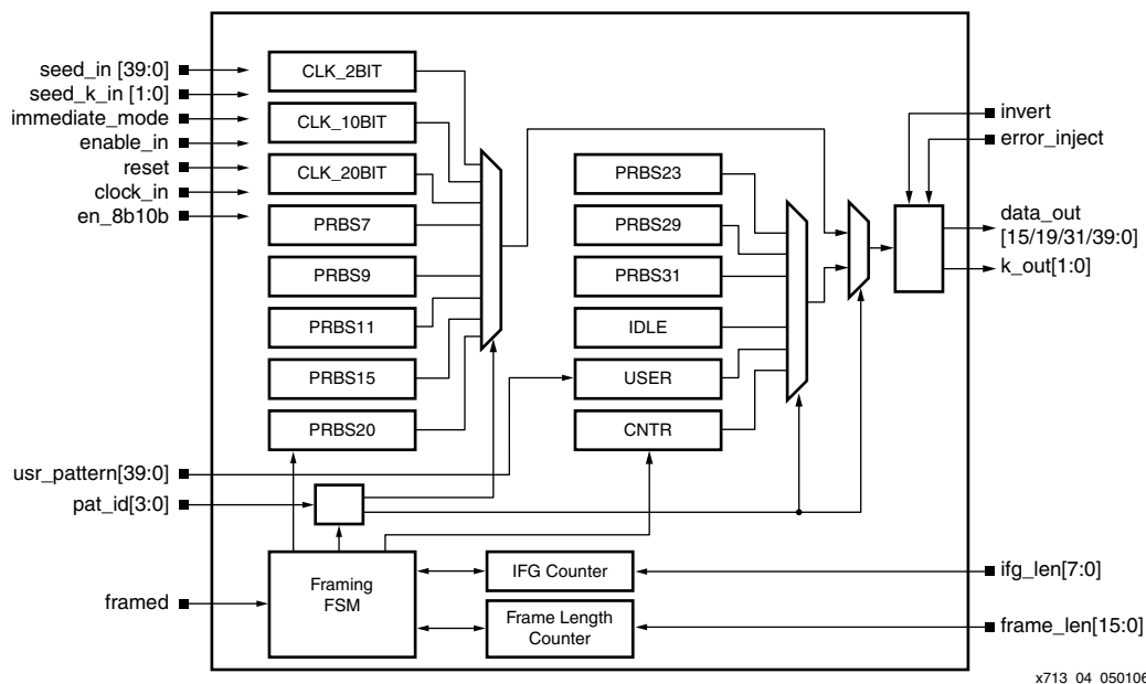
Figure 4: Pattern Generator Block Diagram
