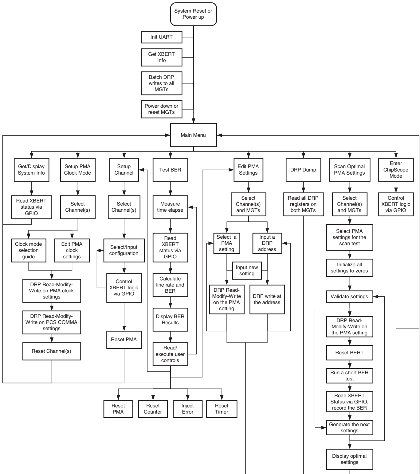
Figure 13: Flow Diagram of Main Application Code
