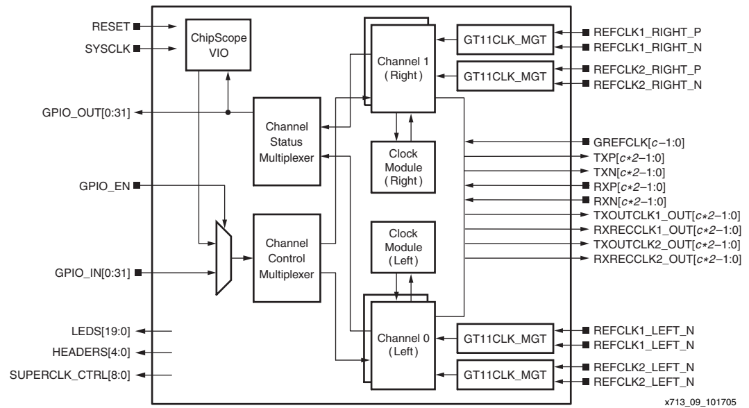
Figure 9: Multi-Channel XBERT Module
