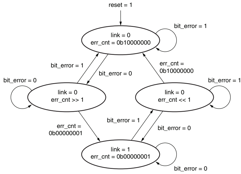
Figure 7: Link Detection State Diagram
