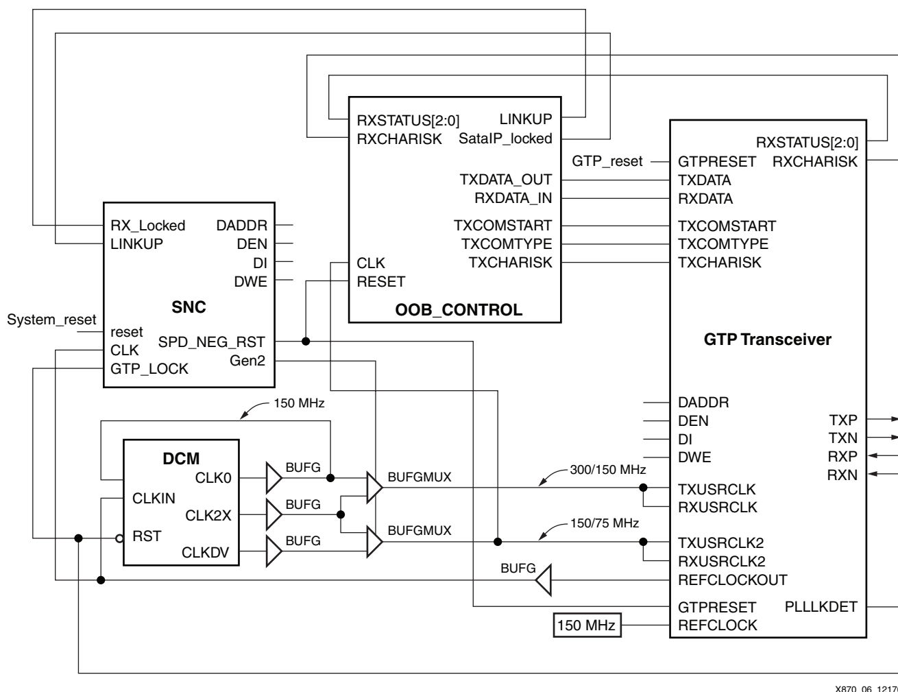
Figure 6: Reference Design Clocking Scheme
