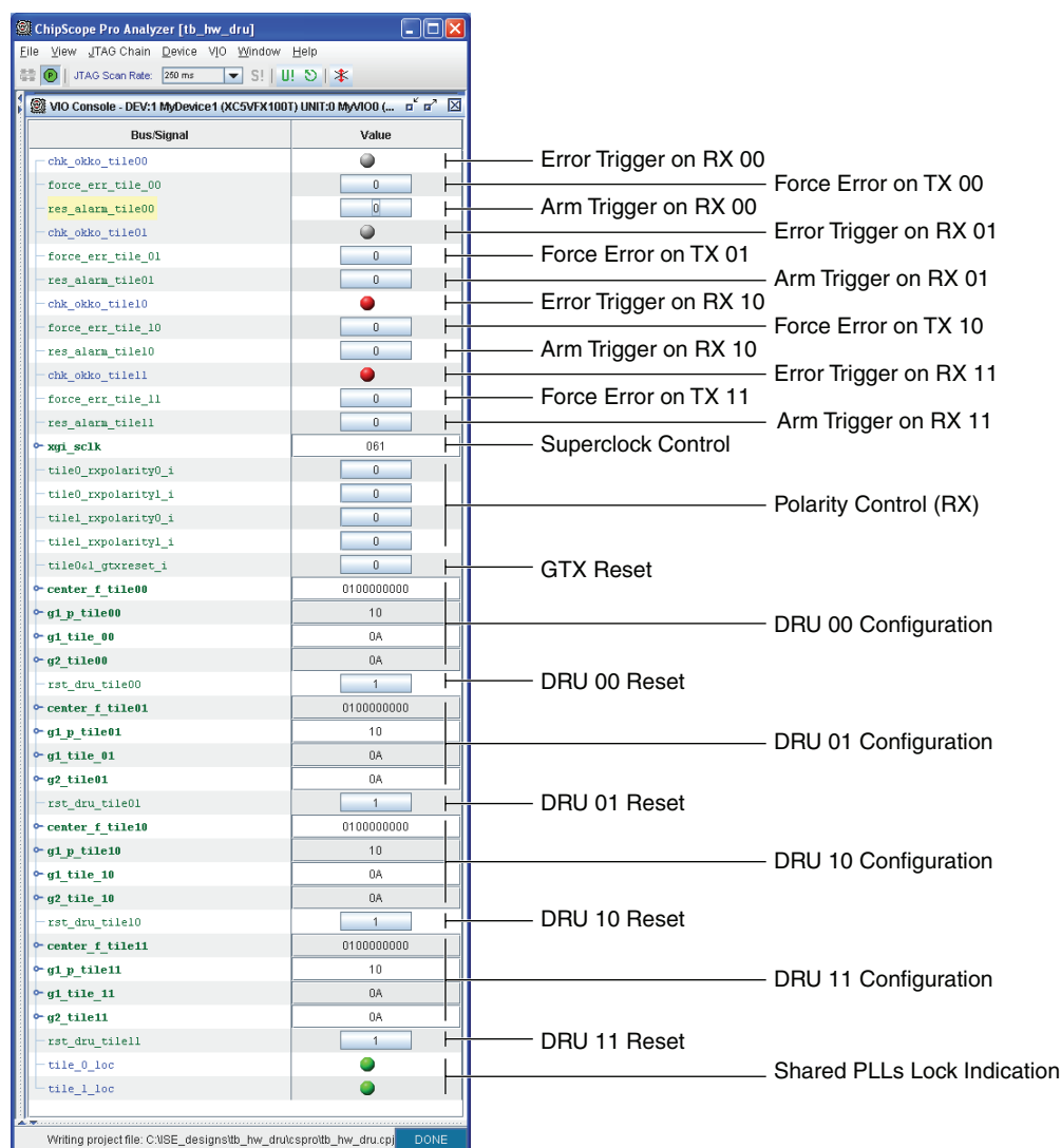
Figure 5: The ChipScope Pro Analyzer Controlling the Demonstration
