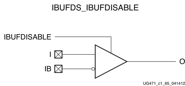
Figure 1-21: Differential Input Buffer With Input Buffer Disable (IBUFDS_IBUFDISABLE)
