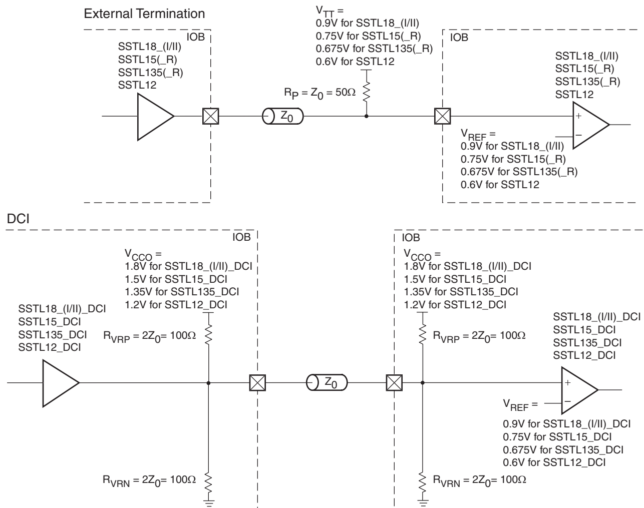
Figure 1-54: SSTL18, SSTL15, SSTL135, or SSTL12 Unidirectional Termination
