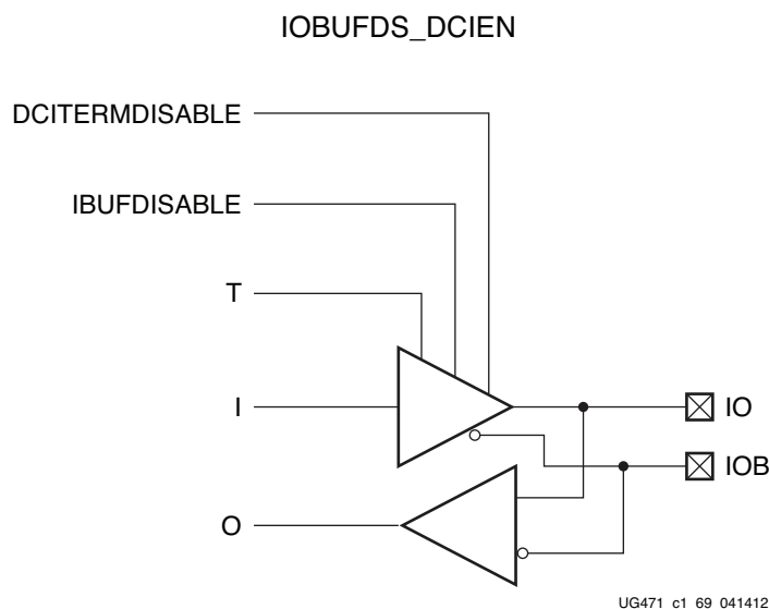
Figure 1-25: Differential Bidirectional Buffer With Input Path Disable and DCI Disable (IOBUFDS_DCIN)
