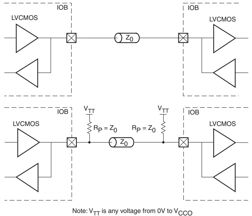
Figure 1-37: LVC MOS Bidirectional Termination
