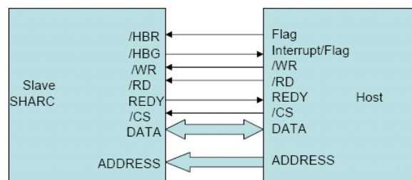
Figure 1. Example: slave mode configuration
