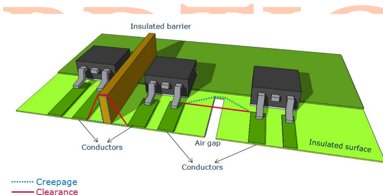
Fig. 3.1: Definition of creepage and clearance
