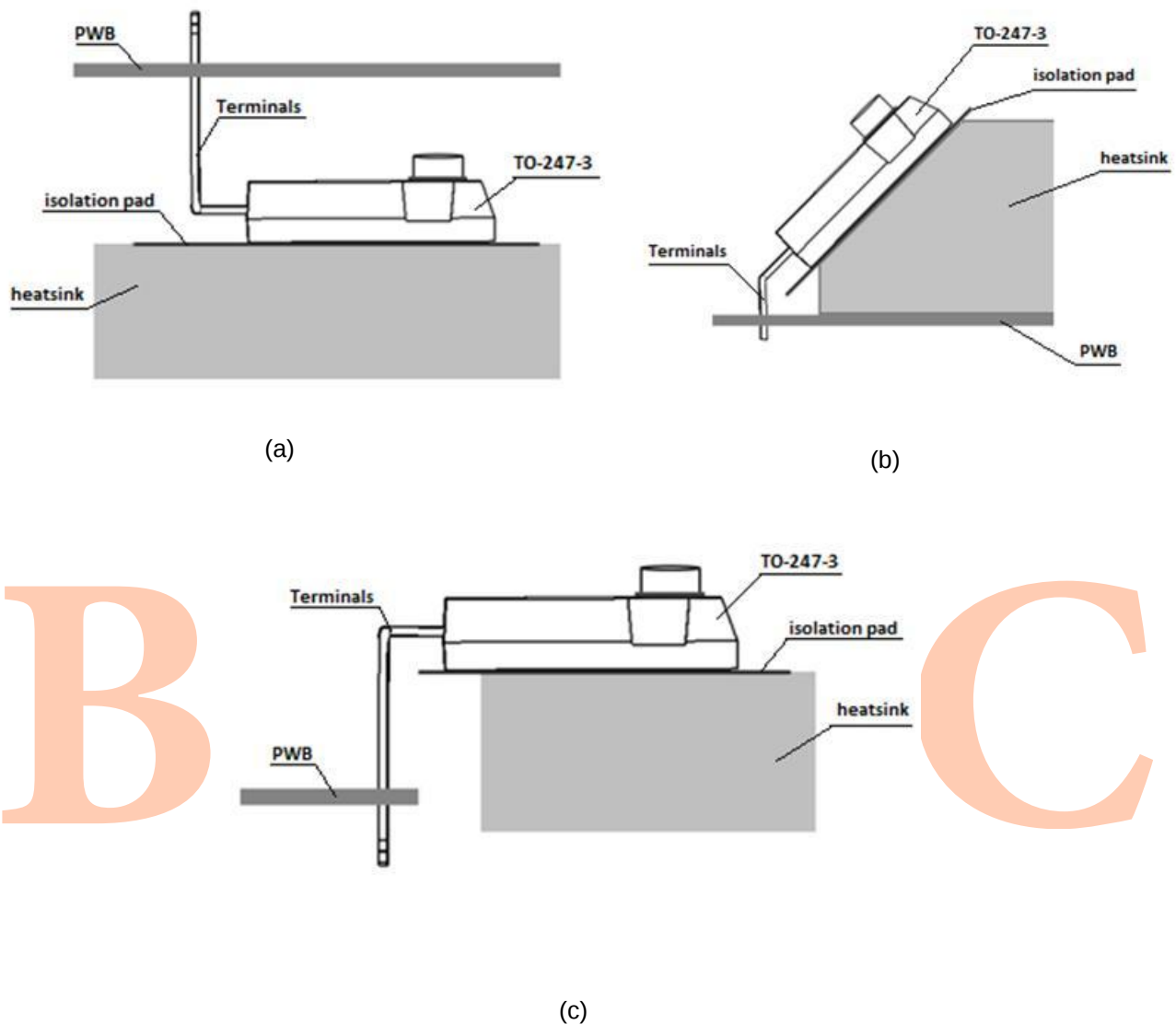
Fig. 4.4: Example of mounting a TO-247-3 with different bending of terminals and different heatsinks.
