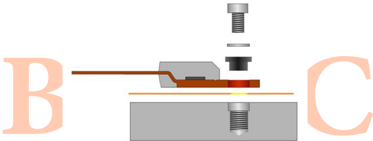
Fig. 4.9: Example of correct assembly of a TO-220 screwed on a heatsink via threatened blind hole
