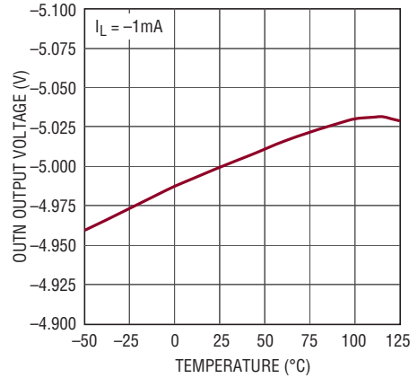
LT3032-5 OUTN Output Voltage
