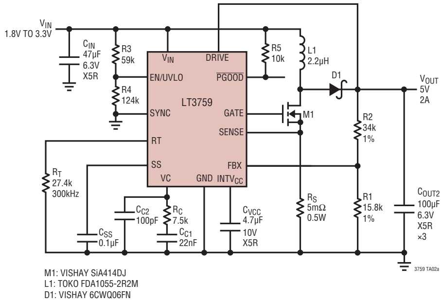
1.8V to 3.3V Input, 5V/2A Output Boost Converter
