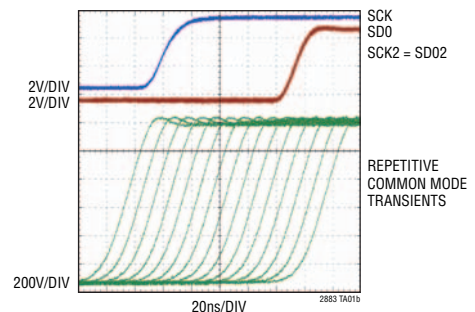
LTM2883 Operating Through 35kV/μs CM Transient
